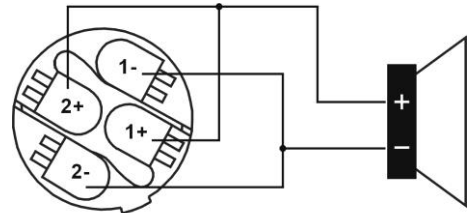
SPEAKON WIRE CONNECTION
